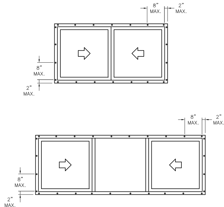
Elevation Views
